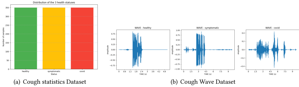
Figure 2. Cough Dataset
